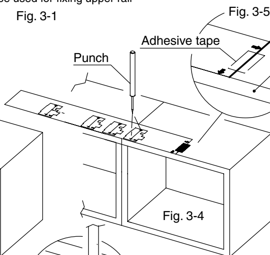
Portion to be used for fixing upper rail
