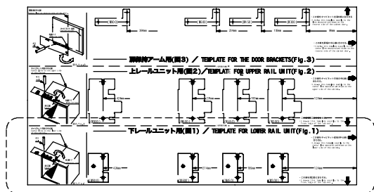
Portion to be used for fixing lower rail
