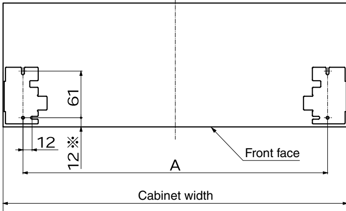
Upper rail ① installation
