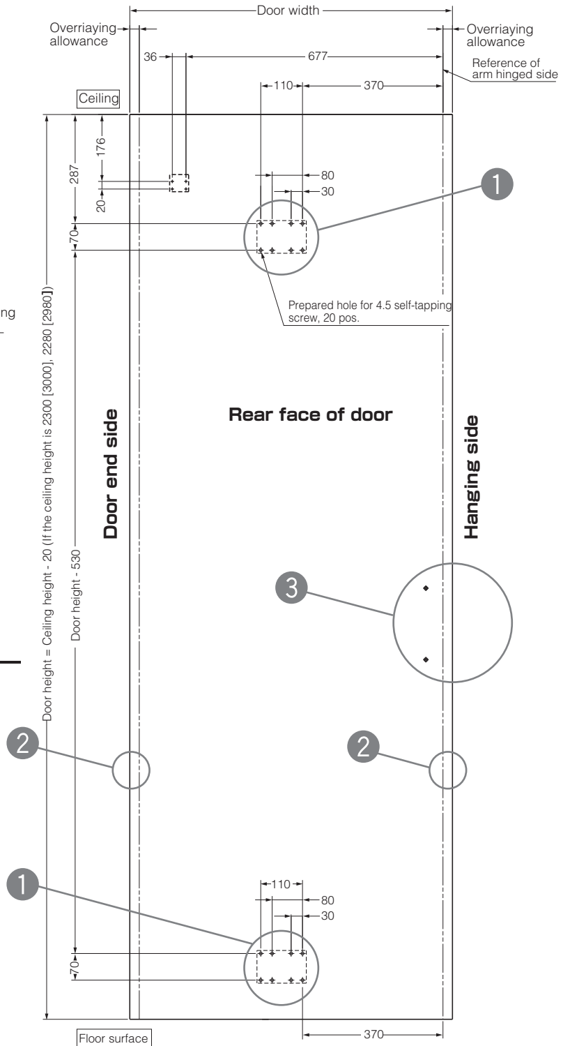
Working dimensional drawing of door
